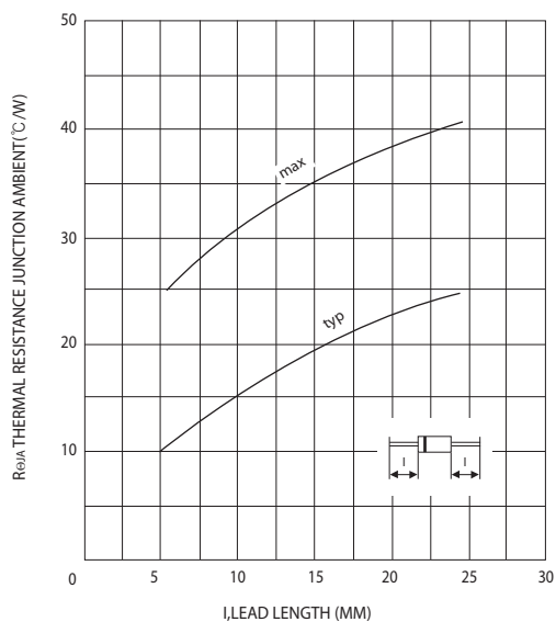
FIG.3-TYPICAL THERMAL IMPEDANCE
